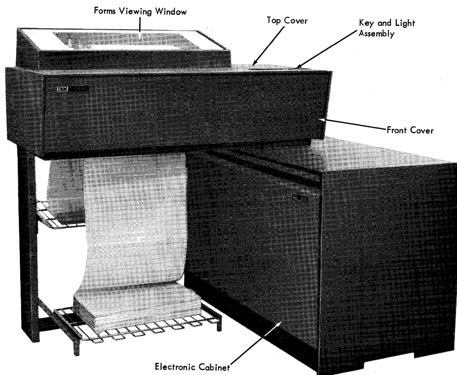
Figure 63. IBM 1443 Printer
