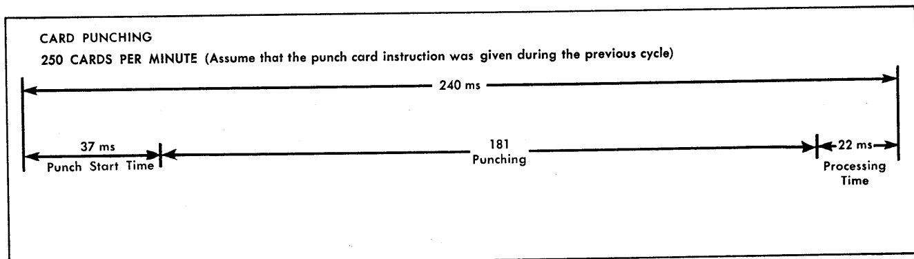
Figure 61. Punch Cycle
