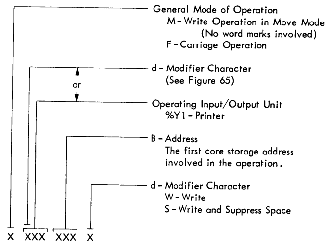
Figure 64. IBM 1443 Printer Instruction Format
